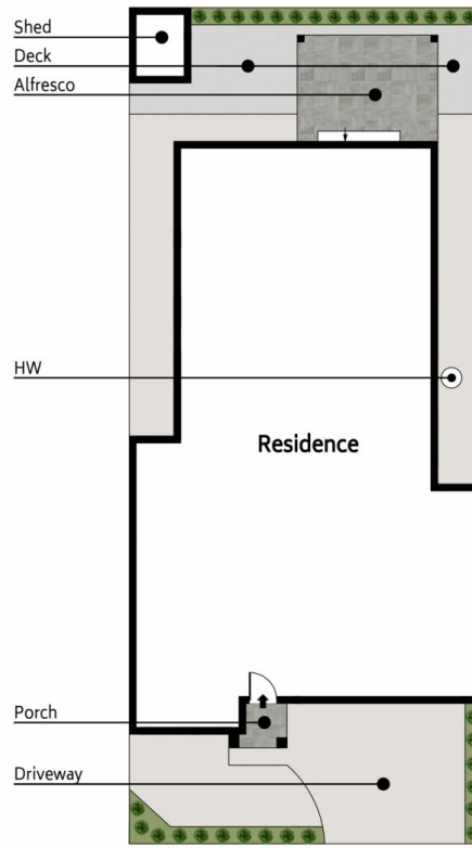
//SITE PLAN
